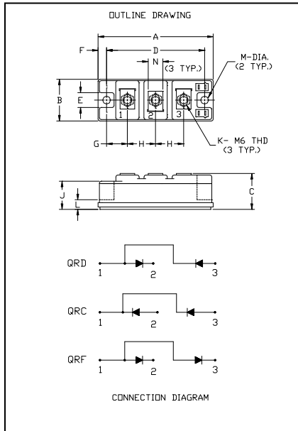
QR_1410T30 Fast Recovery Diode Module
