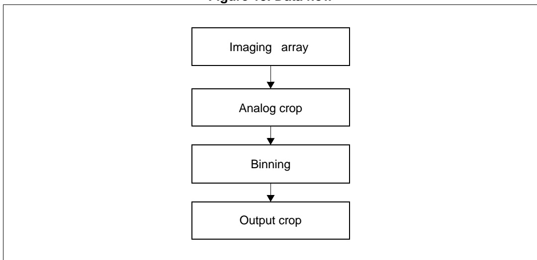
Figure 13. Data flow
