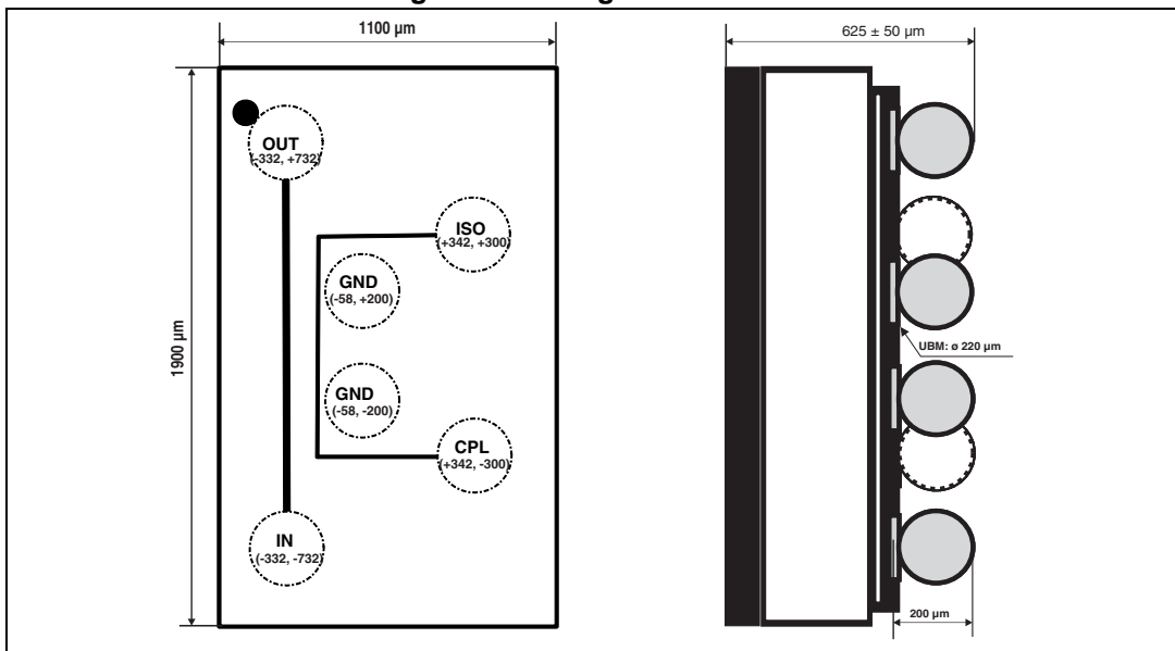
Figure 9. Package dimensions
