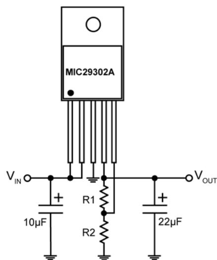
Figure 3. Adjustable Regulator with Resistors
