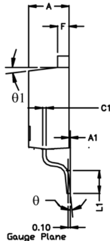
SIDE VIEW 1
