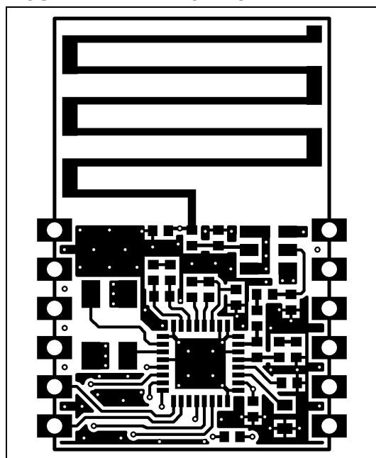
FIGURE 2-4: TOP COPPER
