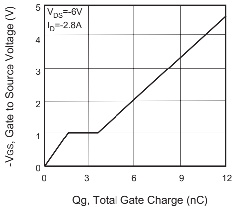
Figure 7. Gate Charge
