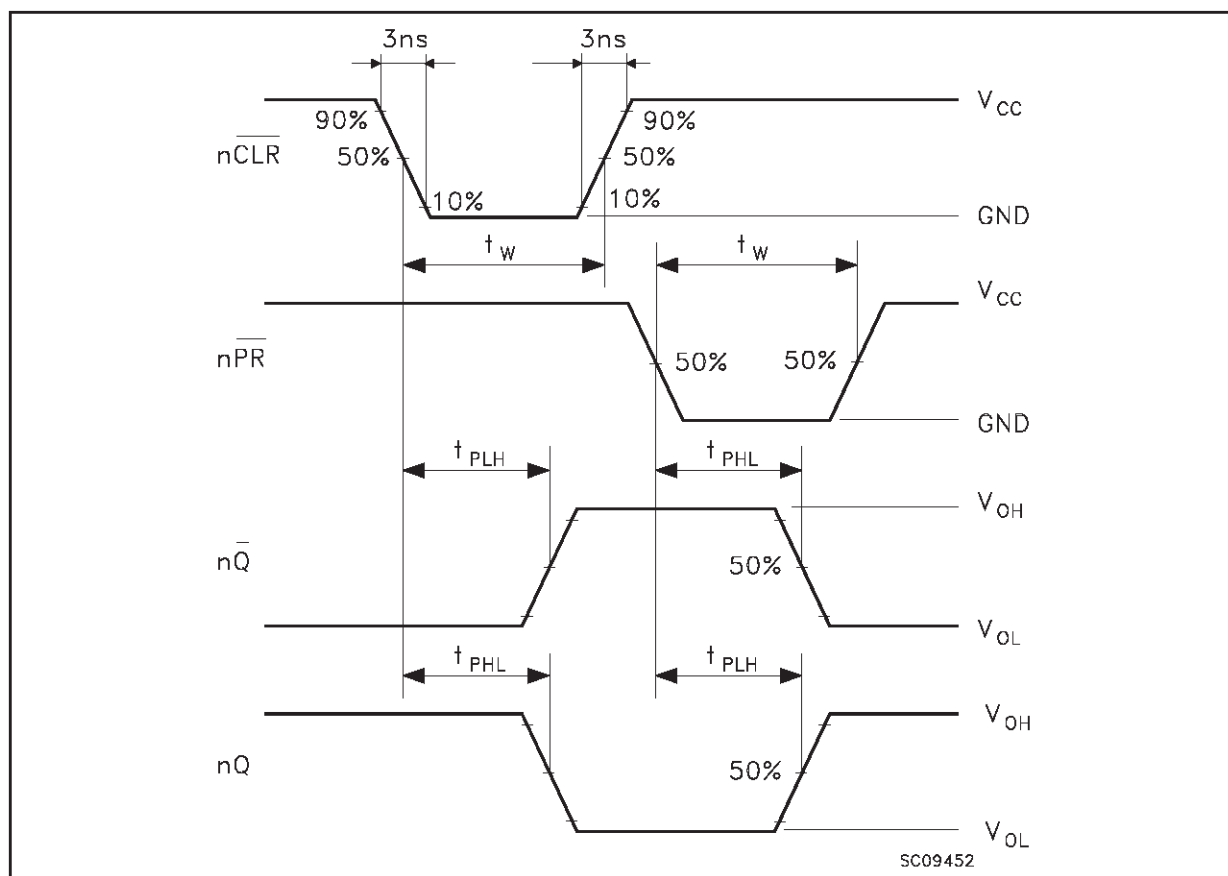
WAVEFORM 3: RECOVERY TIMES ( f=1\text{MHz} ; 50% duty cycle)
