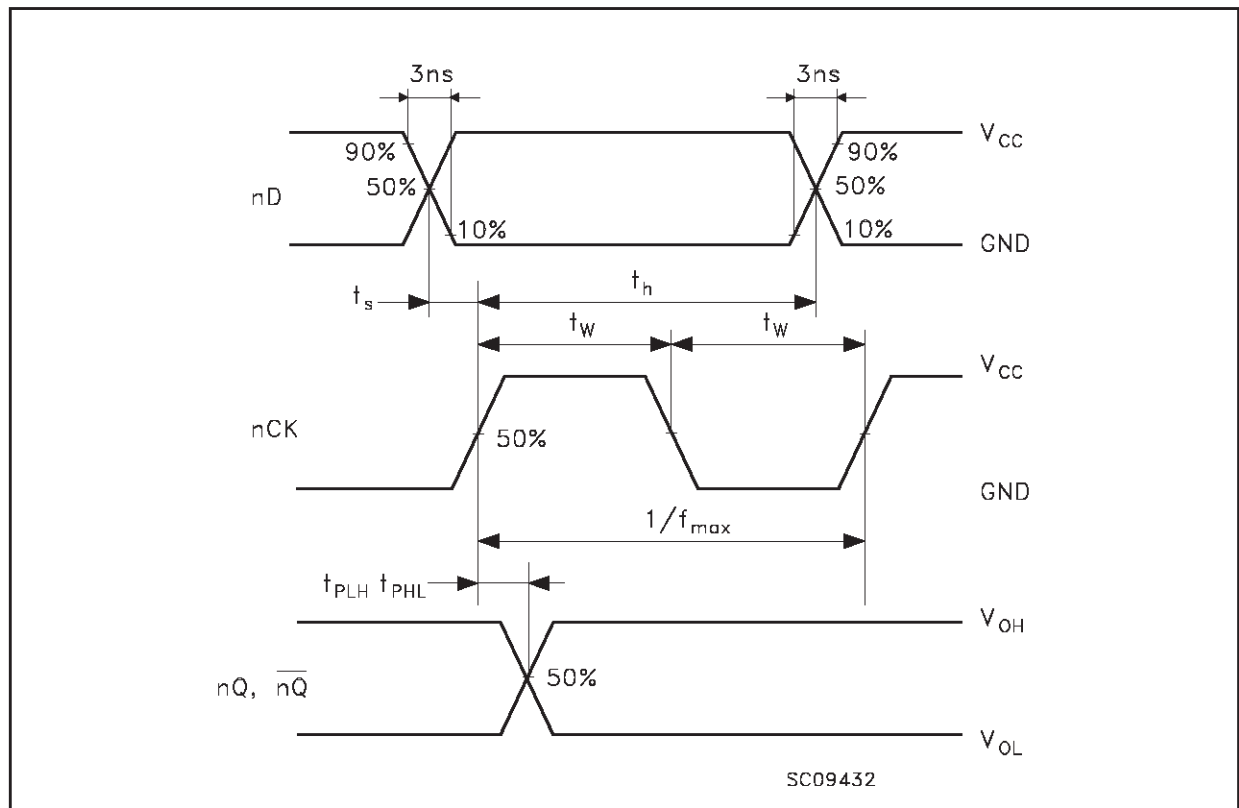
WAVEFORM1:PROPAGATION DELAYS,SETUP AND HOLD TIMES ( f=1\text{MHz} ;50%dutycycle)
