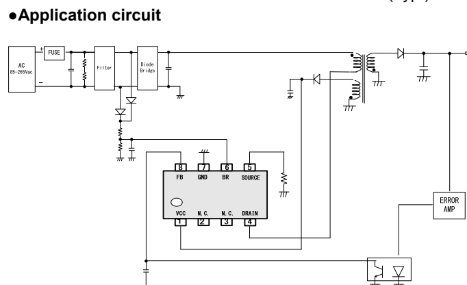
Figure 1. Application circuit
