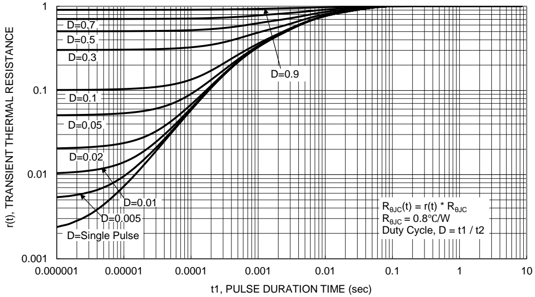
t_1 , PULSE DURATION TIME (sec) Figure 14 Transient Thermal Resistance
