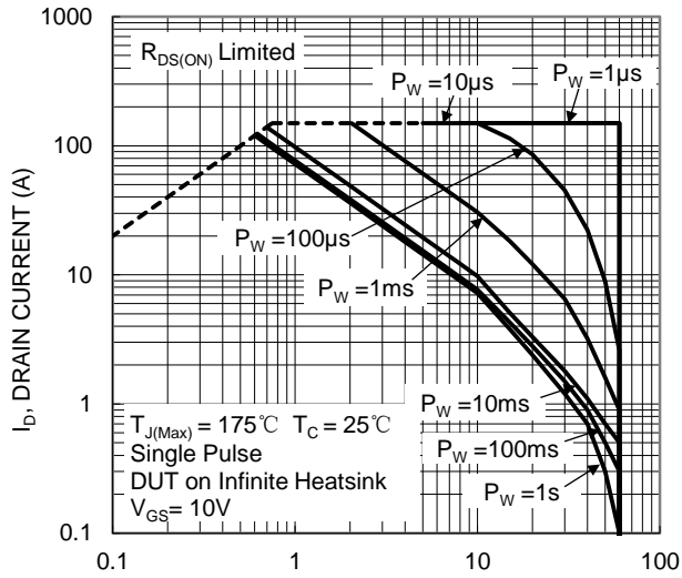
V_{DS} , DRAIN-SOURCE VOLTAGE (V) Figure 13 SOA, Safe Operation Area
