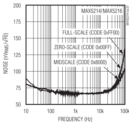
DAC OUTPUT NOISE DENSITY vs. FREQUENCY
