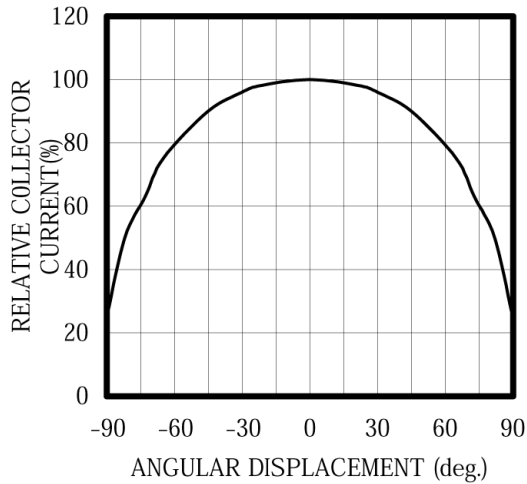
ANGULAR DISPLACEMENT
