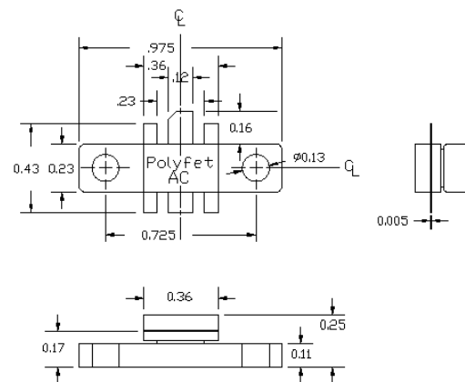
PACKAGE DIMENSIONS IN INCHES
