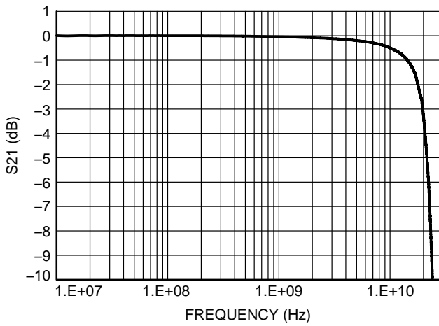
Figure 5. Typical Insertion Loss
