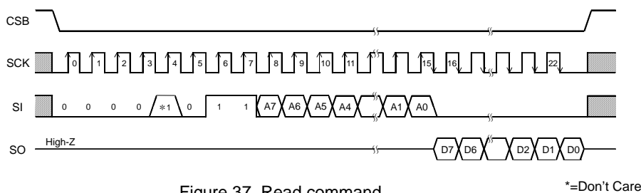
Figure 37. Read command
