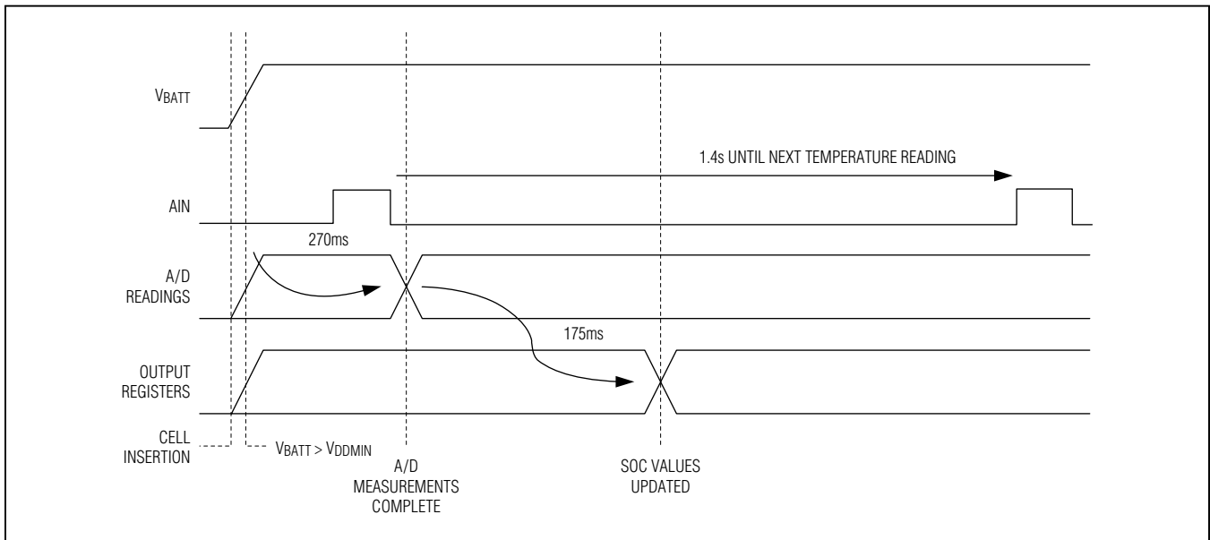
Figure 37. Power-Up Operation
