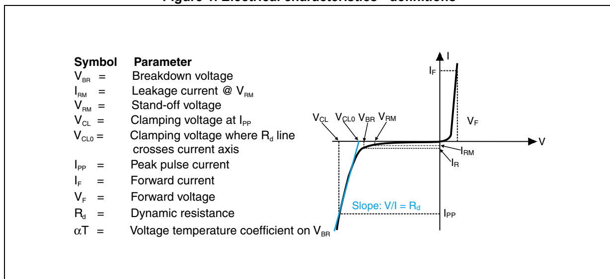
Figure 1. Electrical characteristics - definitions
