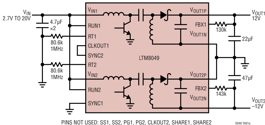
\pm 12V_{OUT} from 2.7V IN to 20V IN
