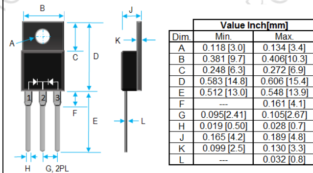
Fig 2. ITO-220AB FOR FR20xxxFCT
