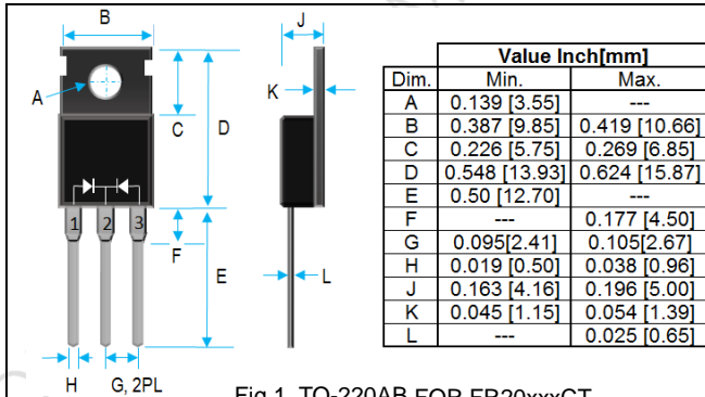
Fig 1. TO-220AB FOR FR20xxxCT
