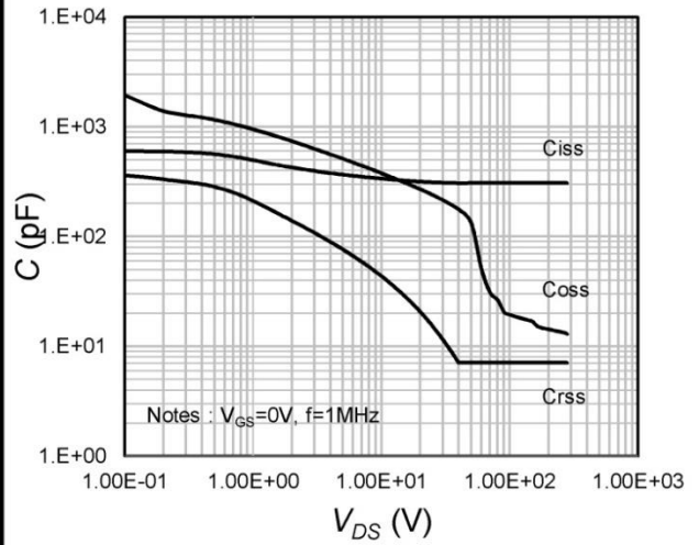
Fig.8 Capacitance Characteristics
