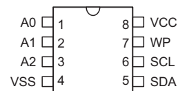
HT24LC128 8 DIP-A/SOP-A/TSSOP-A
