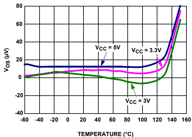
FIGURE 6. PRIMARY V_{SHUNT} V_{OS} vs TEMPERATURE
