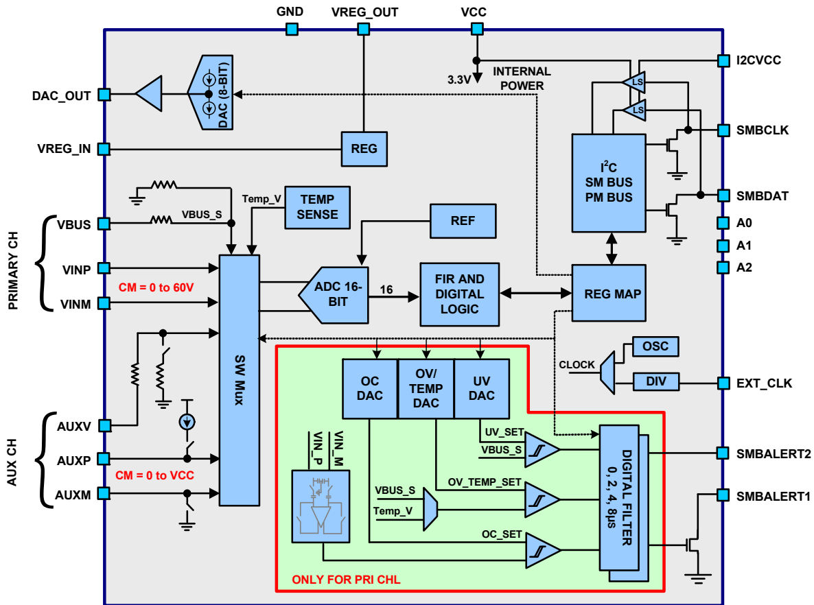
FIGURE 2. BLOCK DIAGRAM
