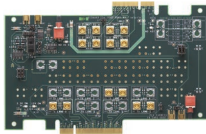
Figure 8. The PCI-SIG Compliance Base Board (CBB2) for Gen2 add-in card testing, and the Compliance Load Board (CLB2) for Gen2 motherboard or host system testing.
