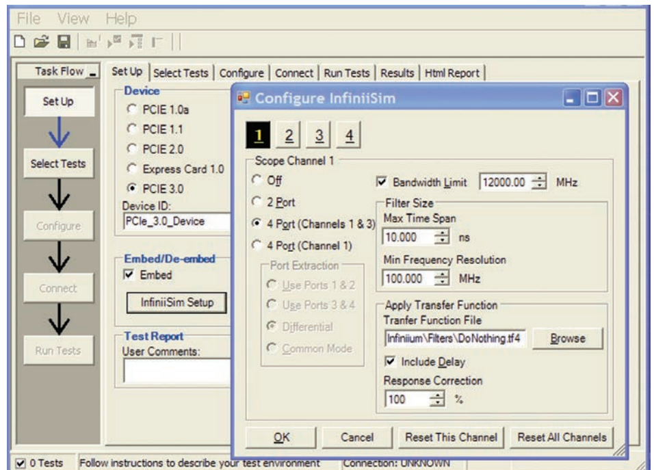
Figure 5. The N5393D integrates de-embedding capability when coupled with the optional InfiniiSim waveform transformation toolset.
