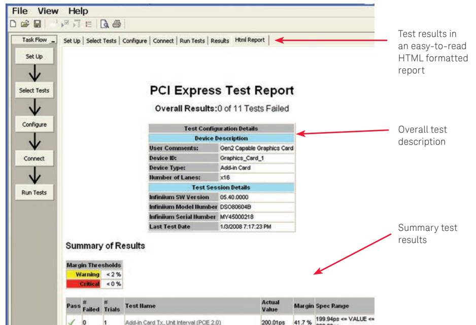
Figure 9. The PCI Express electrical test software results report documents your test, indicates the pass/fail status, the test specification range, the measured values, and shows how much margin you have.
