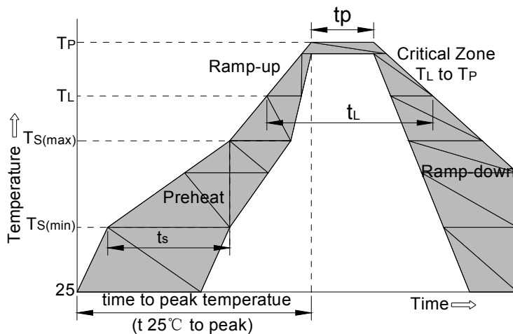
FIG.2: Reflow condition
