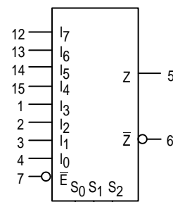
LOGIC SYMBOL
