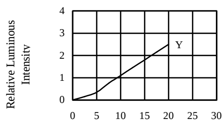
FIG.2-1 RELATIVE LUMINOUS INTENSITY VS. FORWARD CURRENT
