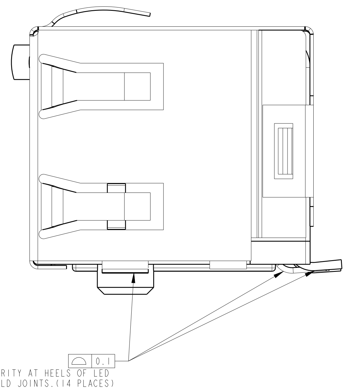
04164 10° TOP VIEW SCALE 4:1
