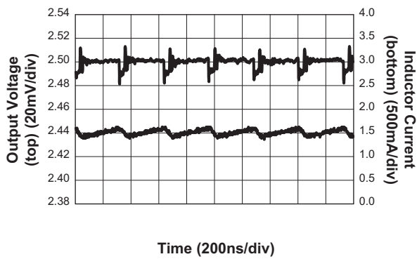
Output Voltage Ripple ( V_{OUT} = 1.8V ; V_{IN} = 3.3V ; I_{OUT} = 1.5A )
