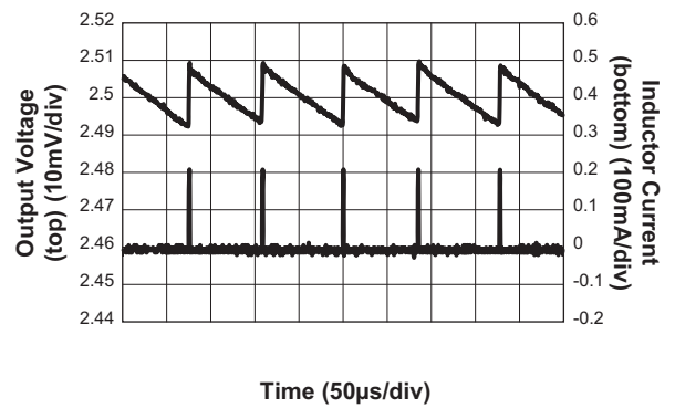
Output Voltage Ripple ( V_{OUT} = 2.5V ; V_{IN} = 3.3V ; I_{OUT} = 1mA )
