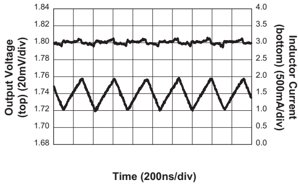
Output Voltage Ripple ( V_{OUT} = 1.8V ; V_{IN} = 3.3V ; I_{OUT} = 1.5A )
