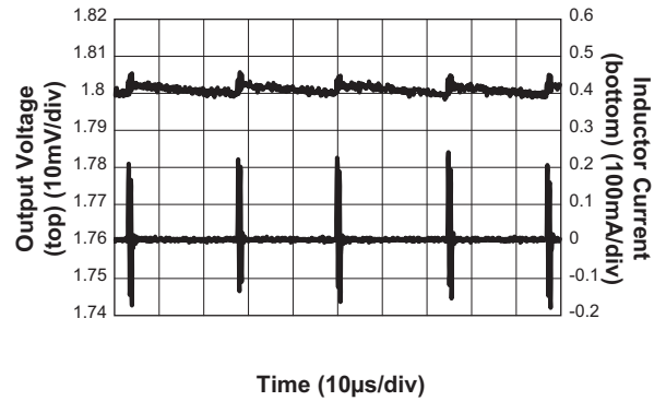
Output Voltage Ripple ( V_{OUT} = 1.8V ; V_{IN} = 3.3V ; I_{OUT} = 1mA )
