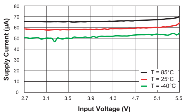
Quiescent Current vs. Input Voltage (No Load)
