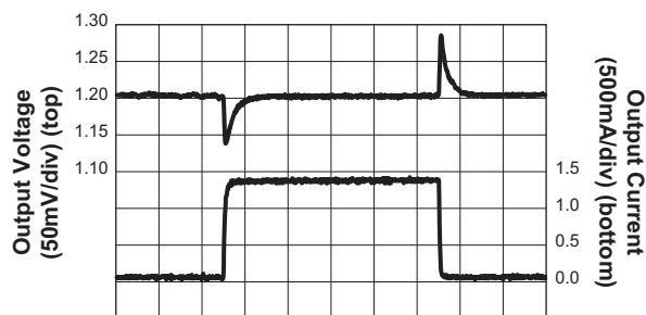
Load Transient
