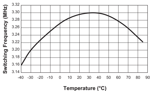
Switching Frequency vs. Temperature ( I_{OUT} = 1A )
