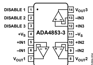
Figure 4. 14-Lead TSSOP
