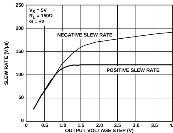
Figure 17. Slew Rate vs. Output Voltage
