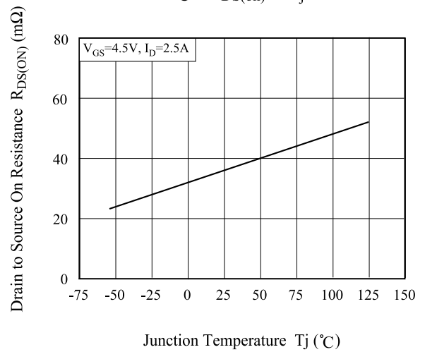
Fig4. R_{DS(on)} - T_j
