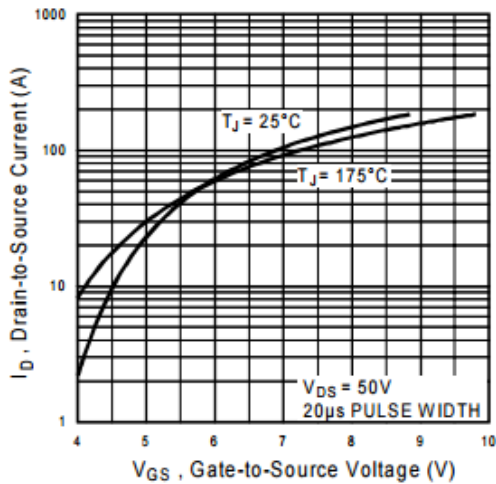
Fig. 3 Typical Output Characteristics, TC = 150^{\circ}C
