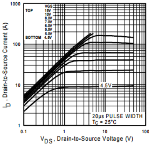
Fig. 1 Typical Output Characteristics, TC = 25^{\circ}
