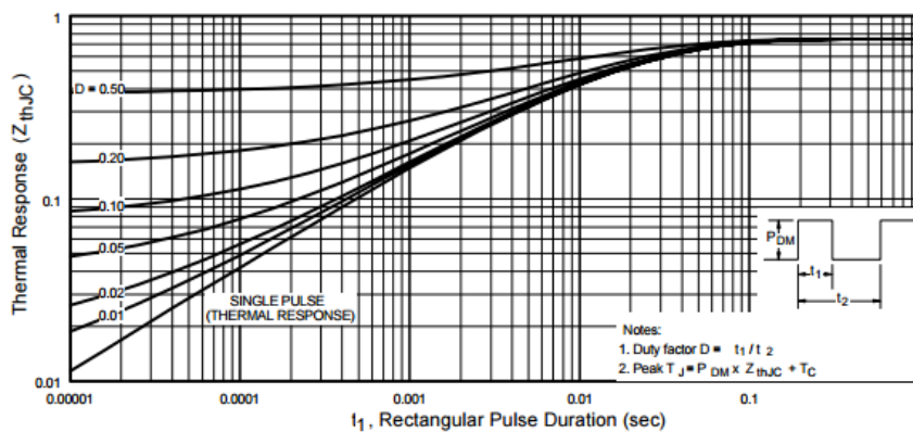
Fig. 9 - Maximum Effective Transient Thermal Impedance, Junction-to-Case
