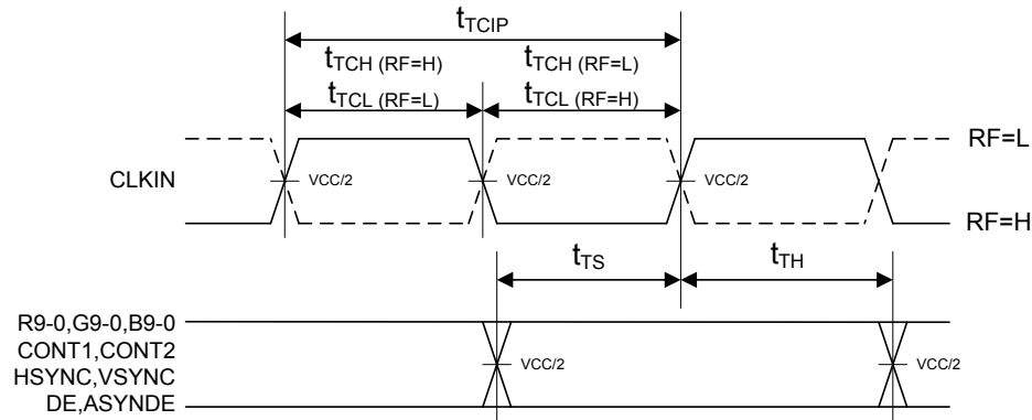
Figure 9. CMOS/TTL Input Switching Timing Diagrams
