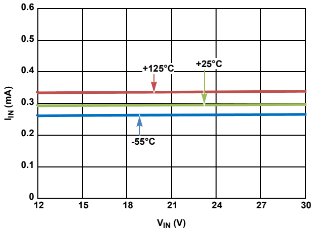
FIGURE 17. I_{IN} vs V_{IN} OVER TEMPERATURE
