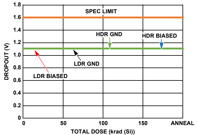
FIGURE 10. DROPOUT SHIFT
