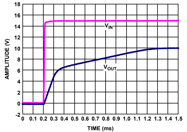
FIGURE 20. TURN-ON TIME
