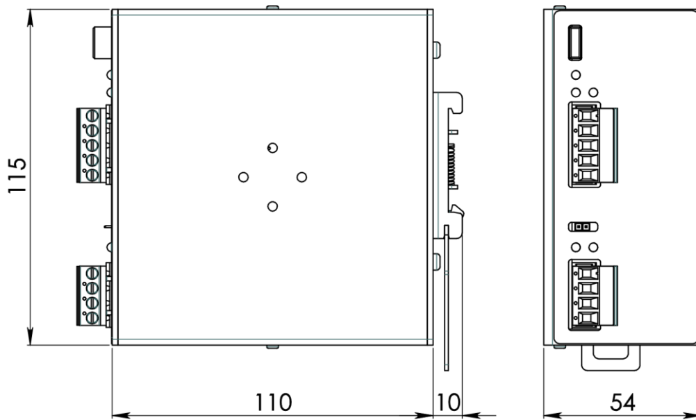
Figure 1. Mechanical Drawing
