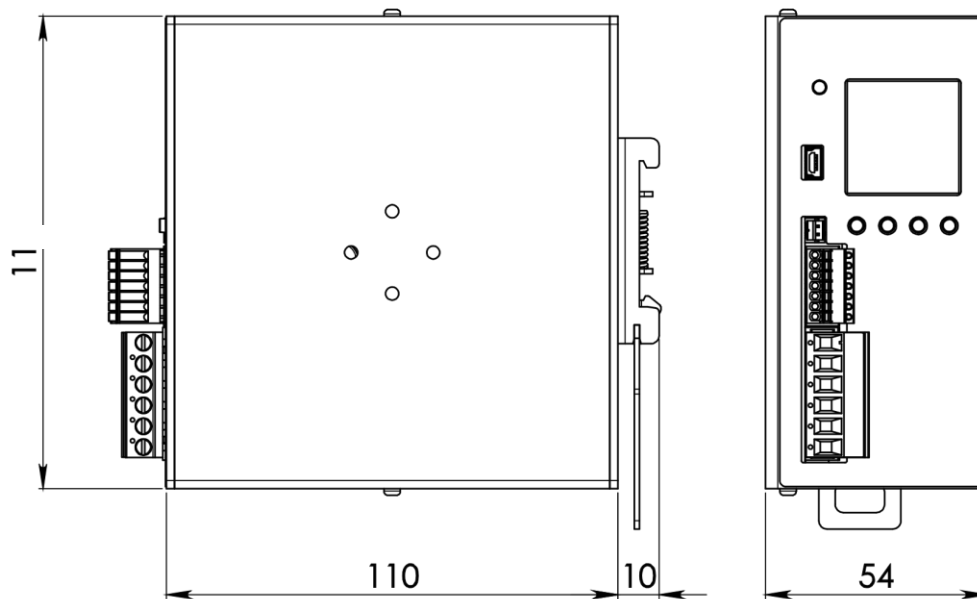
Figure 1. Mechanical Drawing
