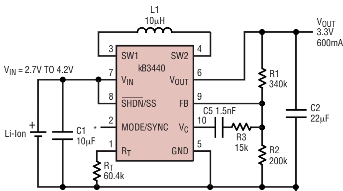
Li-Ion to 3.3V at 600mA Buck-Boost Converter
