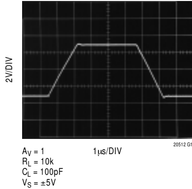
Transient Response
