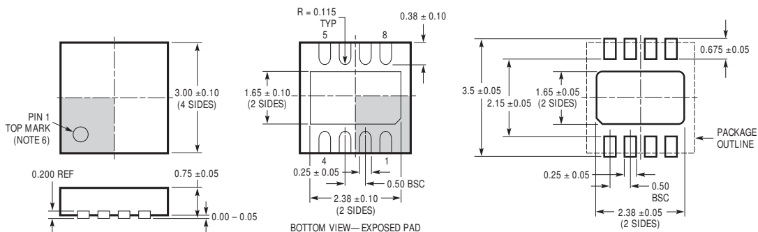
RECOMMENDED SOLDER PAD PITCH AND DIMENSIONS (00) DFN 1203
