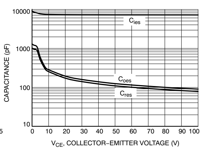
Figure 6. Typical Capacitance
