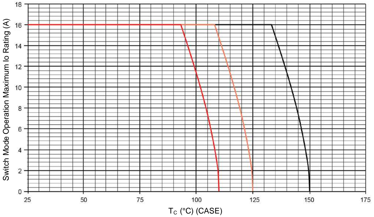
FIGURE 1 Temperature-Current Derating
