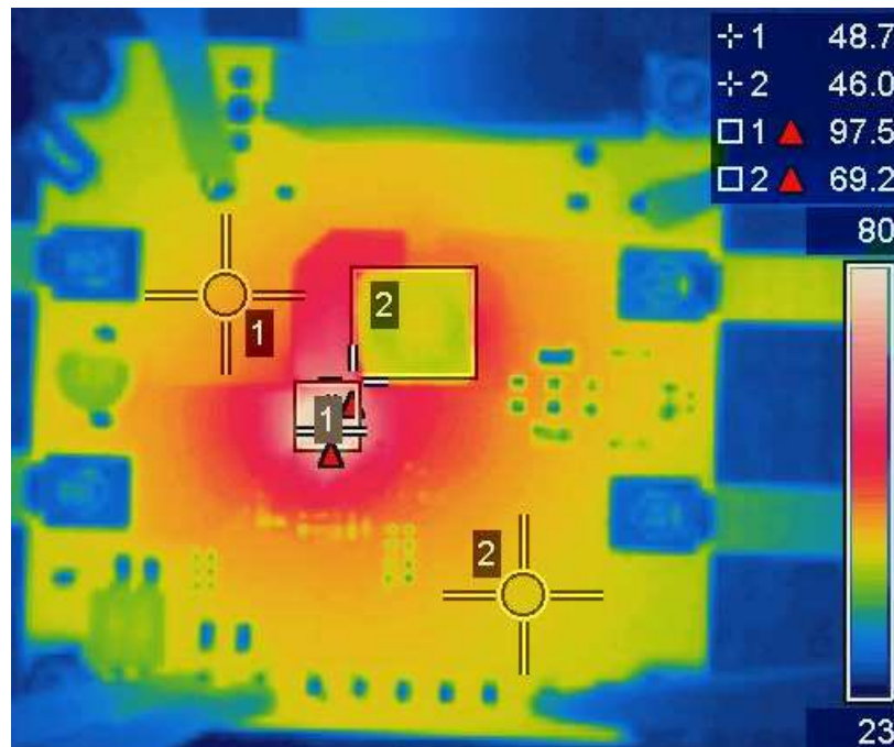
Fig. 17: Thermal Image (IR3477: 98^\circ C , Inductor: 69^\circ C , PCB: 49^\circ C )
