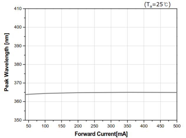
4. Peak Wavelength VS Forward Current
