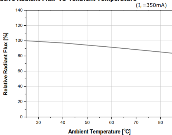
5. Relative Radiant Flux VS Ambient Temperature
