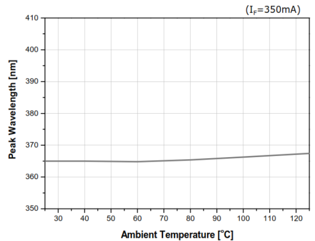
6. Peak Wavelength VS Ambient Temperature
