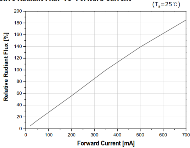
3. Relative Radiant Flux VS Forward Current
