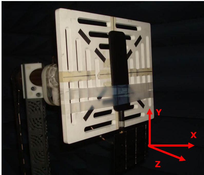
Antenna bent 90° with 90*150mm ground plane
