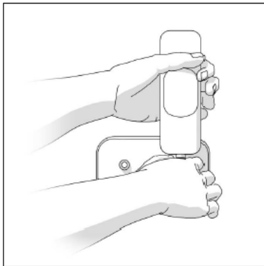
Figure 1. Place the TG.35 antenna onto the connector of the device and hold the antenna in the preferred orientation.
