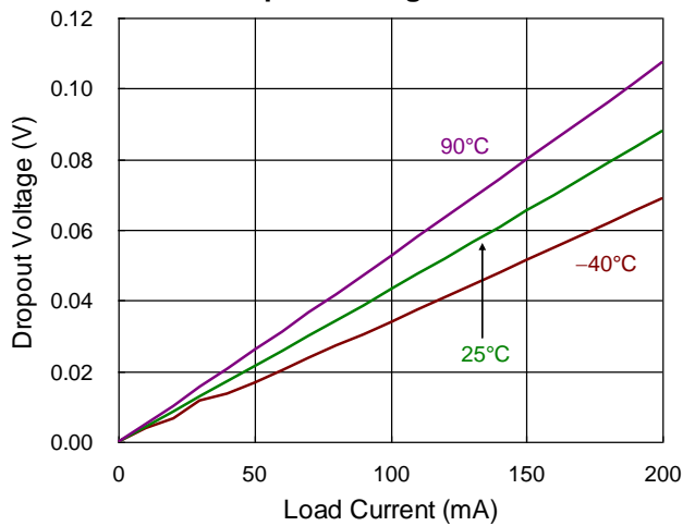
CH6 LDO Dropout Voltage vs. Load Current
