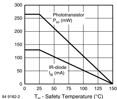
Fig. 3 - Derating Diagram
