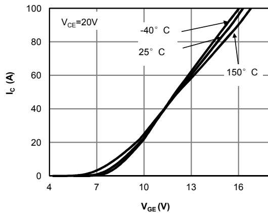
Figure 3: Transfer Characteristic
