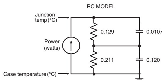
FIGURE 24b. TRANSIENT THERMAL IMPEDANCE MODEL
