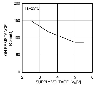
Fig.12 ON resistance
