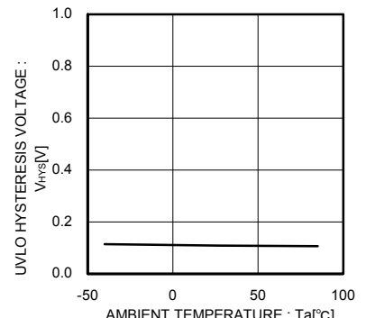
Fig.27 UVLO hysteresis voltage
