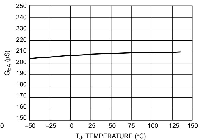
Figure 34. Error Amplifier Gain versus Temperature
