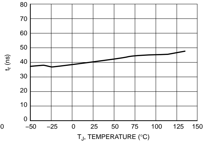
Figure 32. Gate Drive Rise Time versus Temperature
