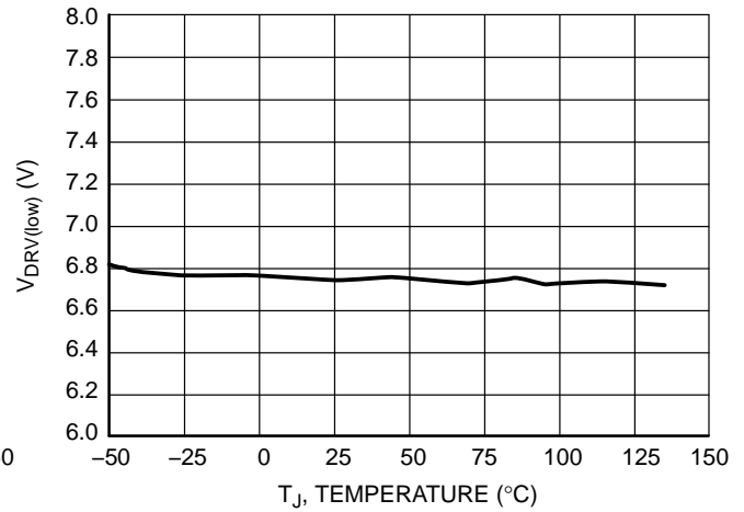
Figure 30. V DRV(low) versus Temperature
