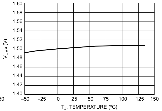
Figure 20. Output Under Voltage Level versus Temperature
