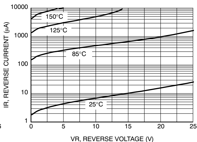
Figure 2. Leakage Current
