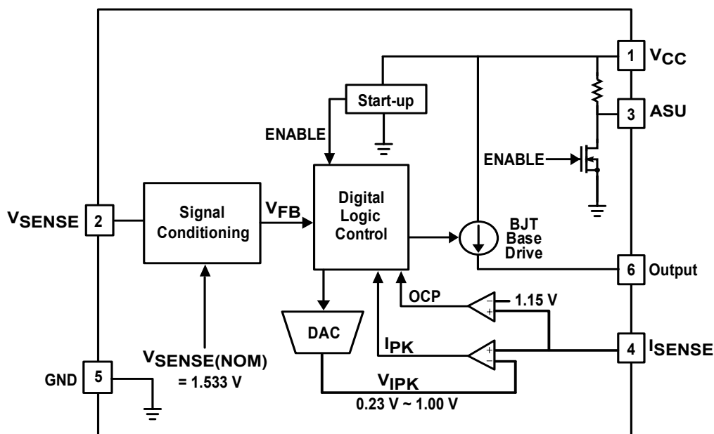
Figure 8.1: iW1707 Functional Block Diagram
