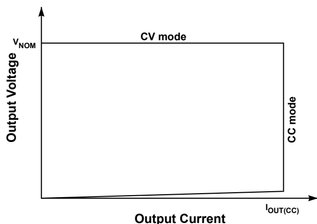
Figure 9.4: Power Envelope
