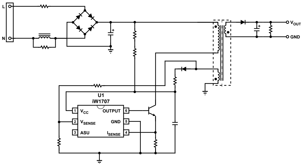
Figure 3.3: iW1707 Alternate Application Circuit without Active Start-up Device
