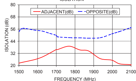
ZC16PD-1900W+ ISOLATION
