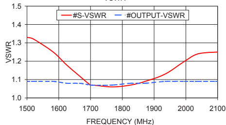
ZC16PD-1900W+ VSWR
